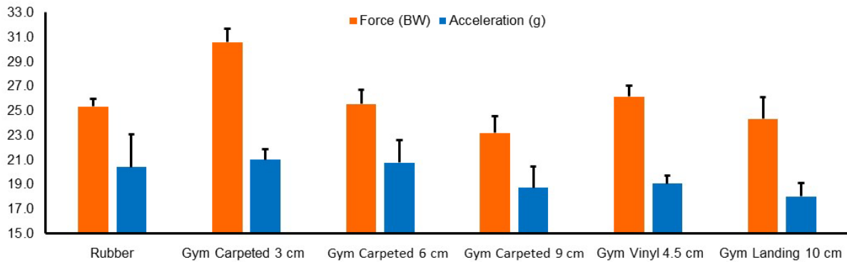
Figure 2: Peak resultant acceleration and ground reaction force for the 60 cm drop height and the viscoelastic sport surfaces.
