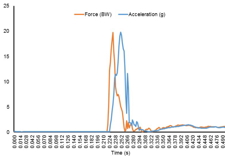
Figure 3: Example force and acceleration-time curves from the force platform and IMU measuring tools. Note that the two measuring tools were not time synchronised.
