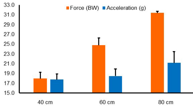
Figure 1: Peak resultant acceleration and ground reaction force for the standard force platform surface testing from three drop heights. Abbreviations: BW is the normalised peak resultant impact force with respect to Body Weights, and g is the normalised peak resultant acceleration with respect to the gravitational constant of -9.81 \text{ m/s}^2 .
